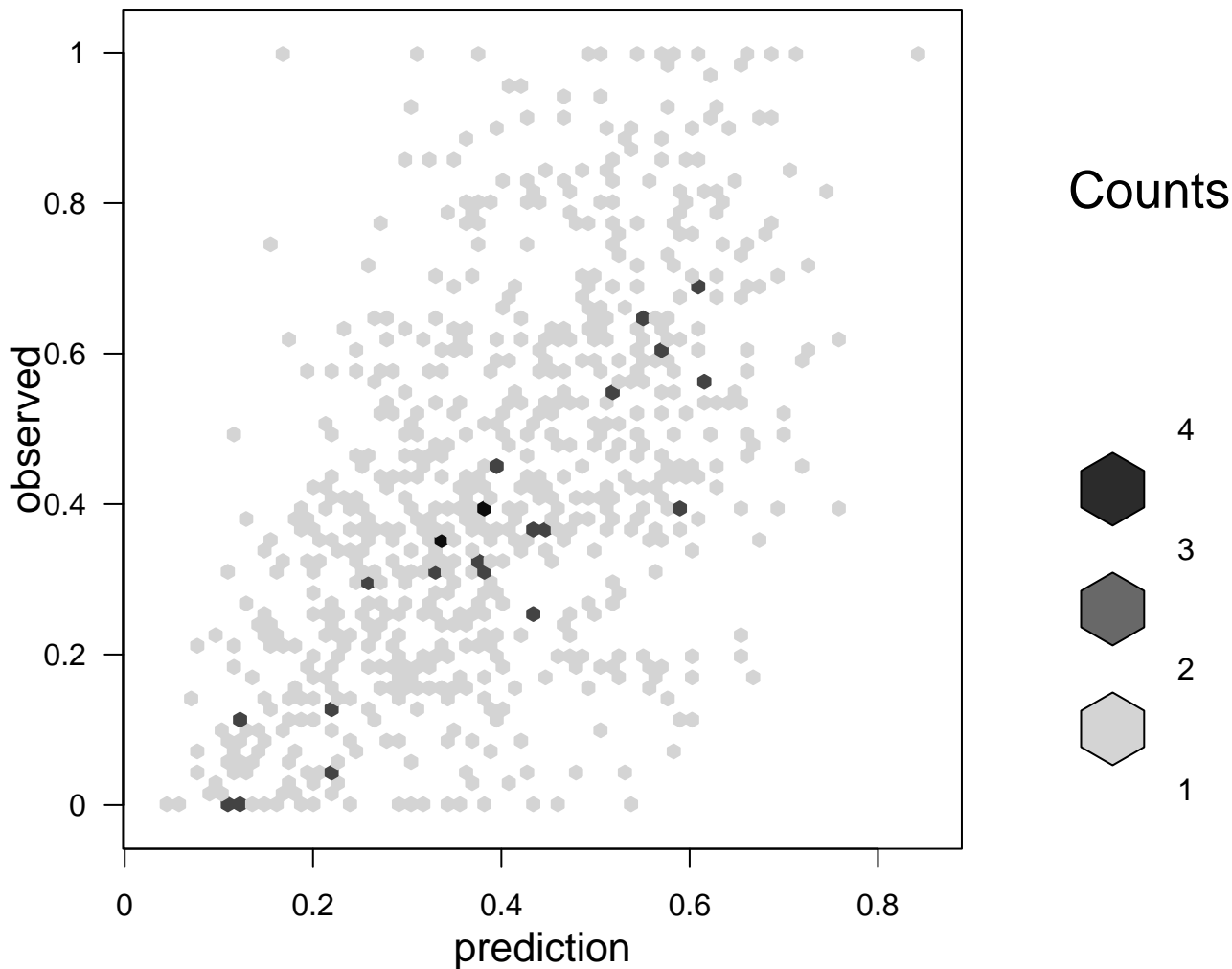
Corr. scatterplot – motif length=9 (800 datapoints)
