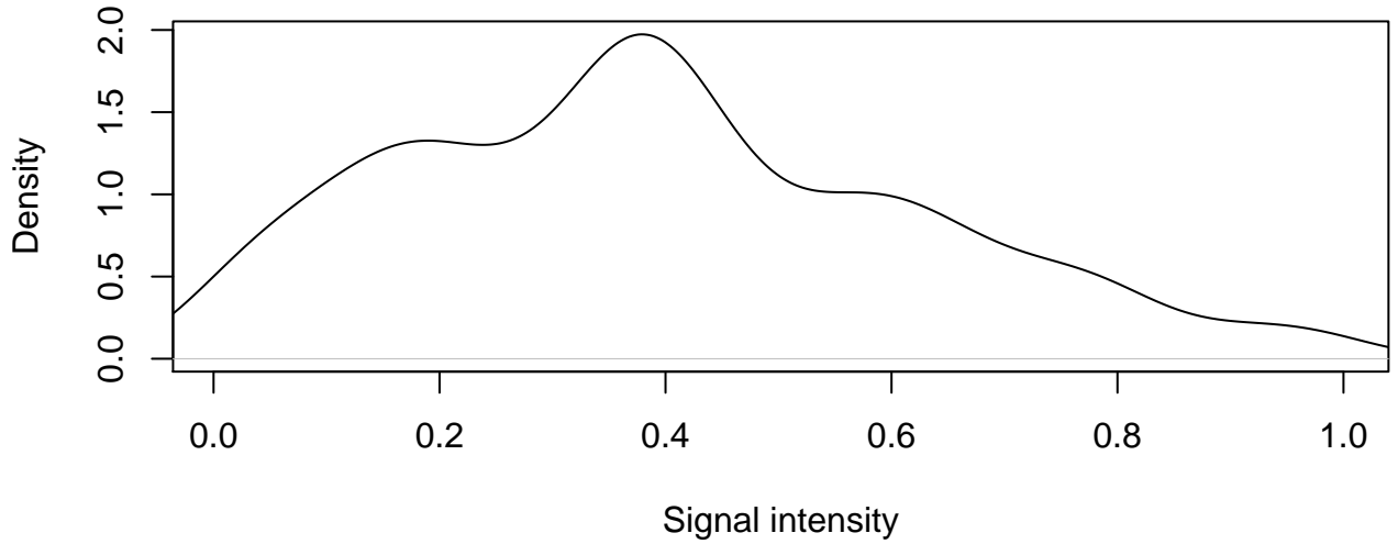
Raw data distribution
