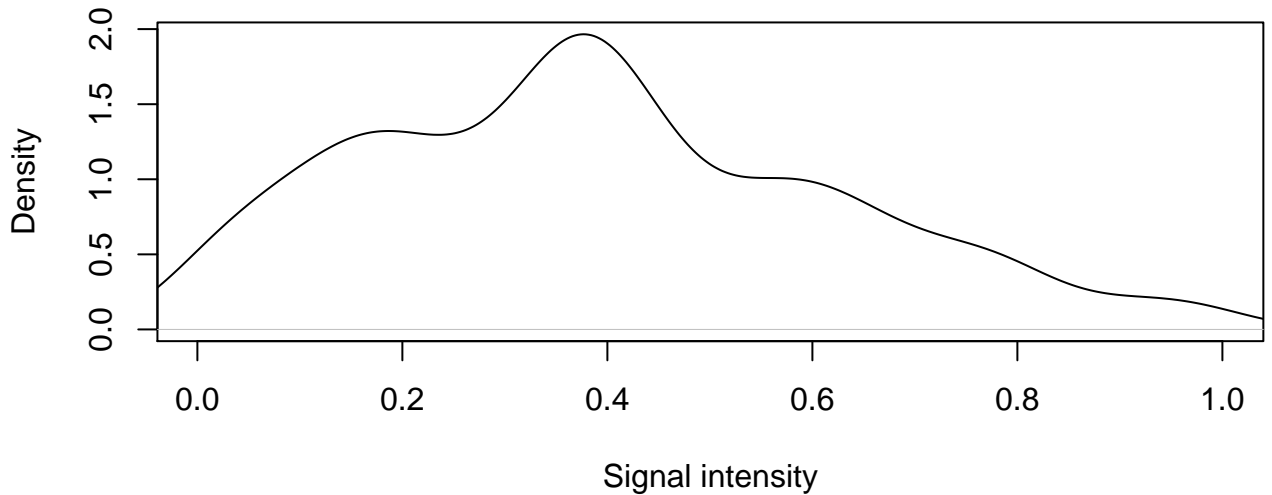
Data distribution after rescaling
