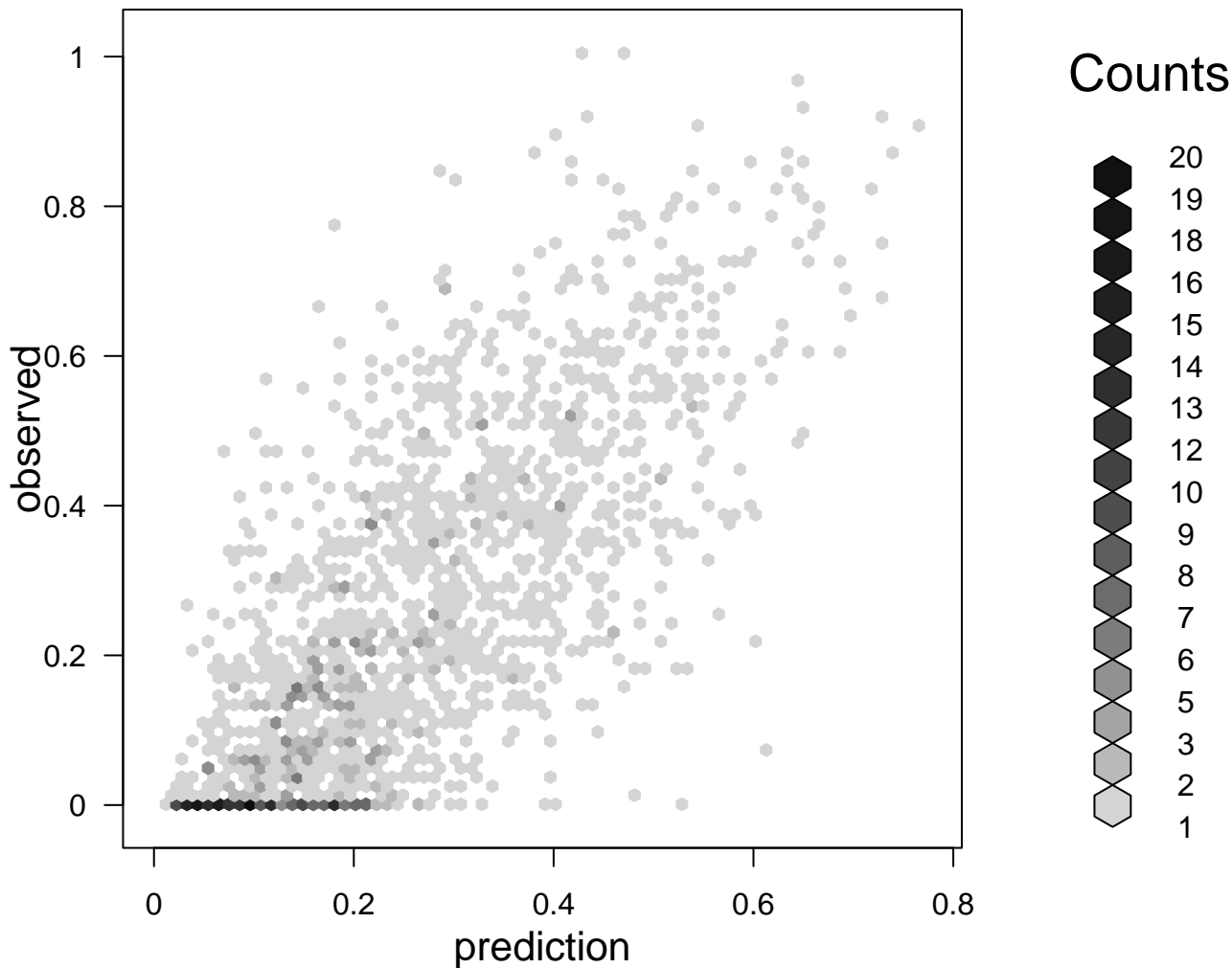
Corr. scatterplot – motif length=9 (1715 datapoints)
